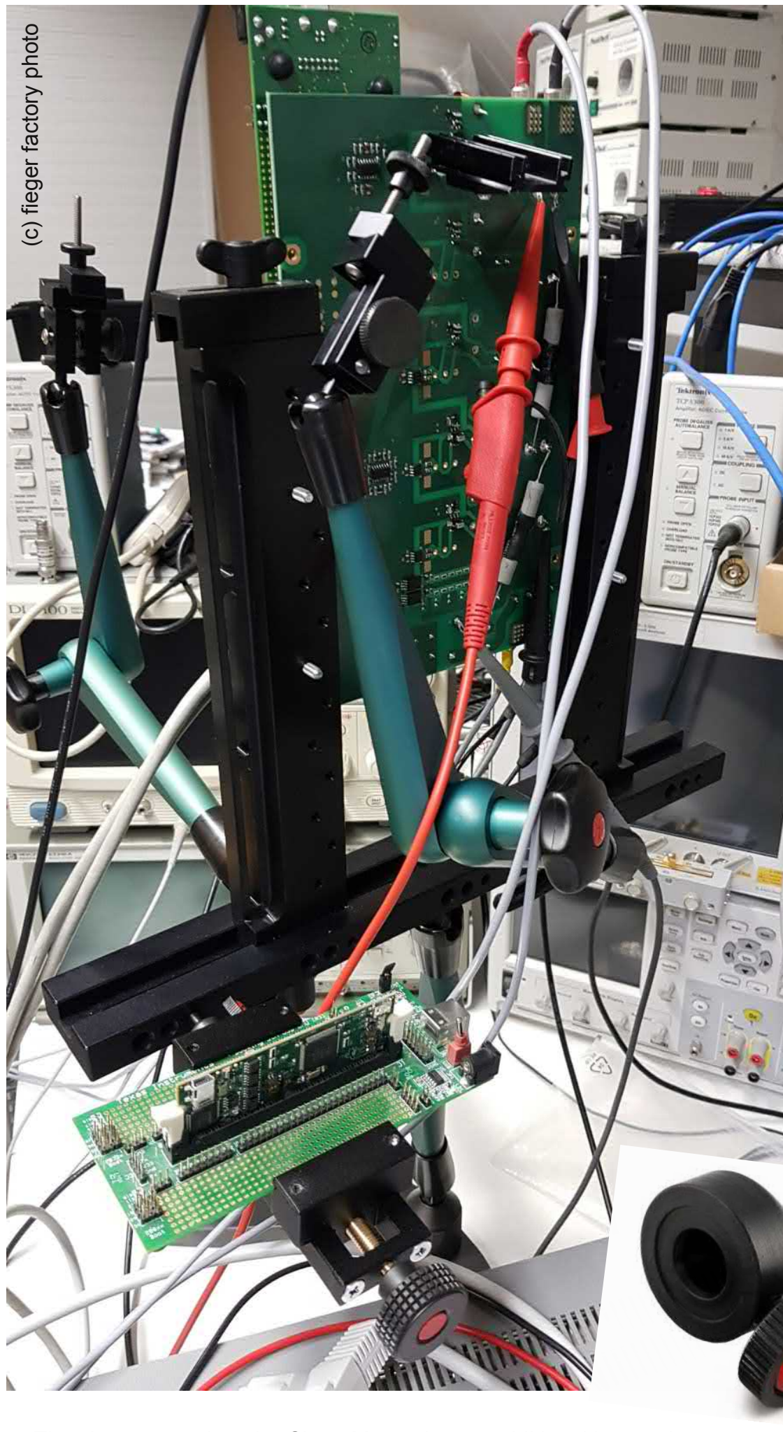
The vice mounted on the ClampMan using an additional base adapter
