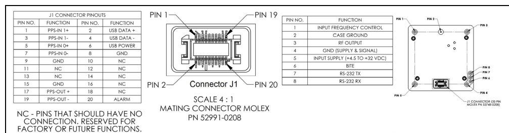
FIGURE 2-3: Pinout.
