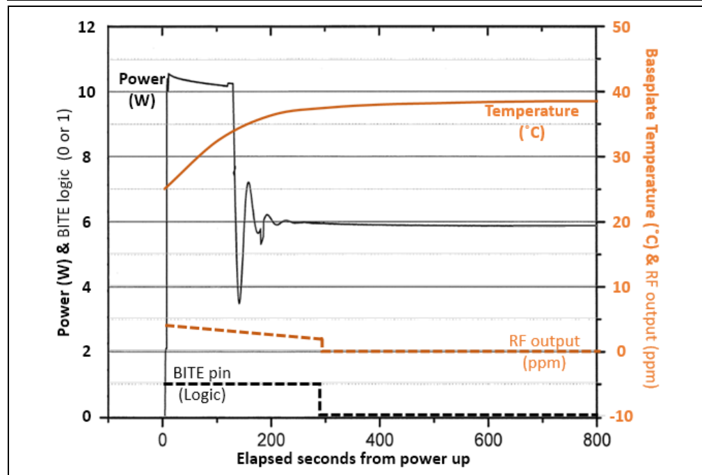
FIGURE 2-4: Start-Up Sequence.
