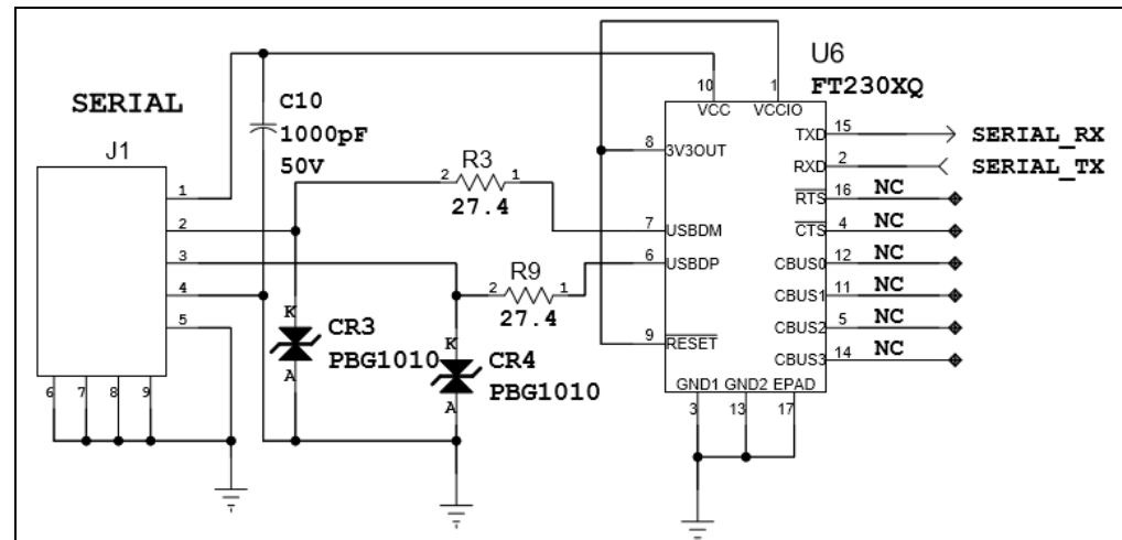
FIGURE C-2: RS-232 Schematic.
