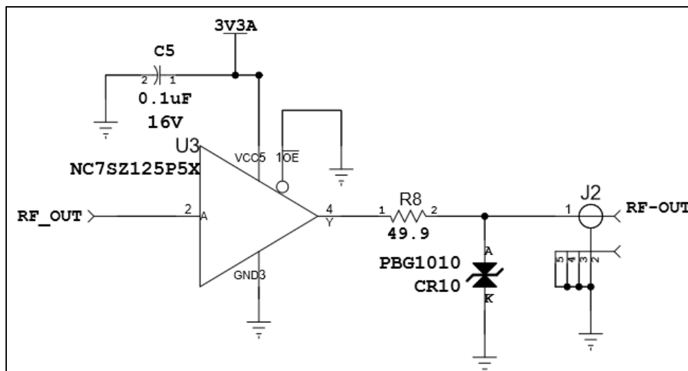
FIGURE C-7: RF Output Schematic.
